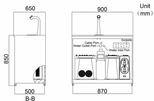
Cabinet Dimensions
